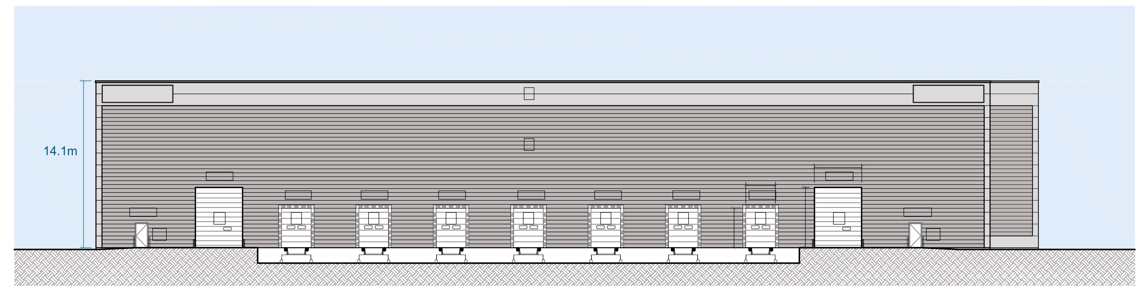
West Elevation
