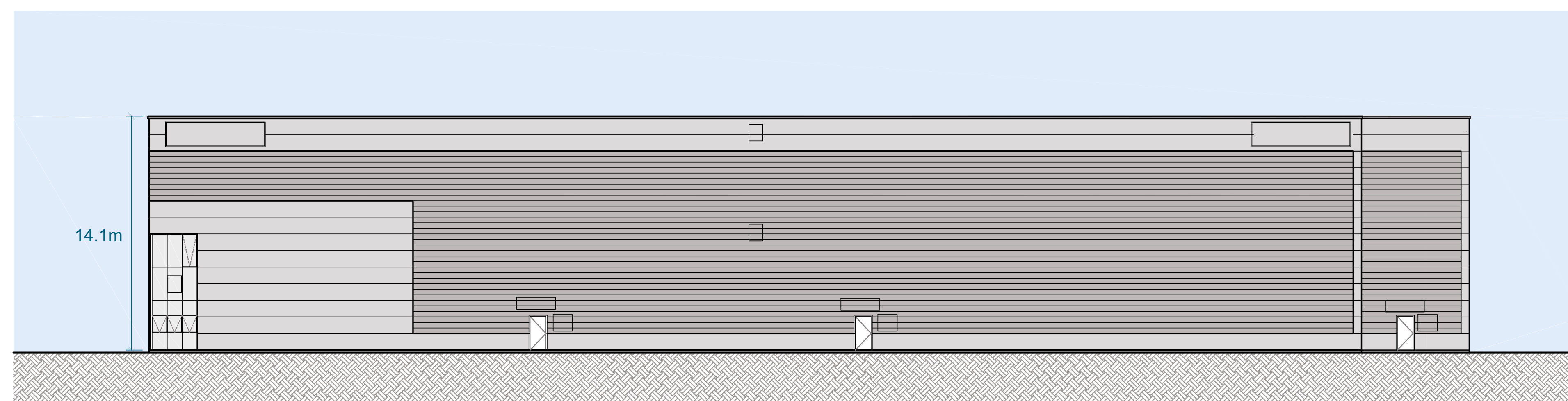
East Elevation
