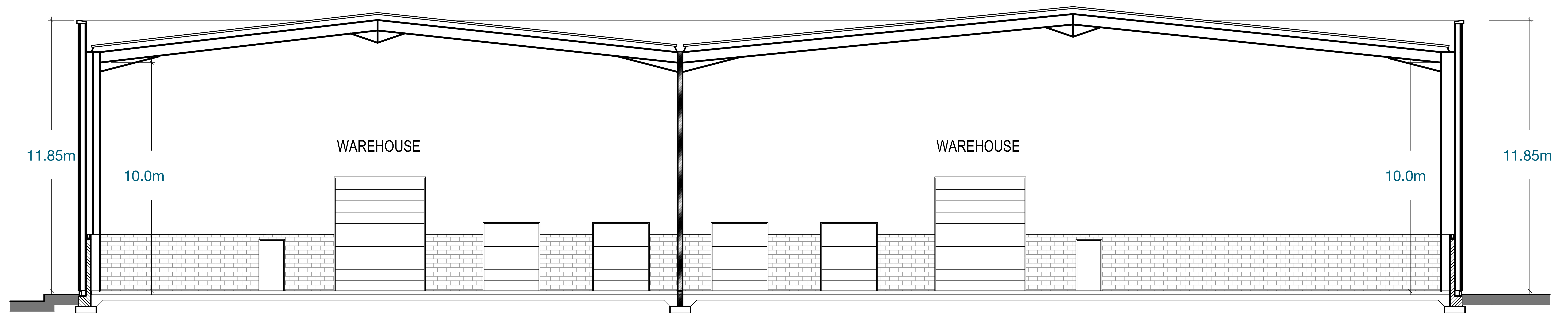
CROSS SECTION
