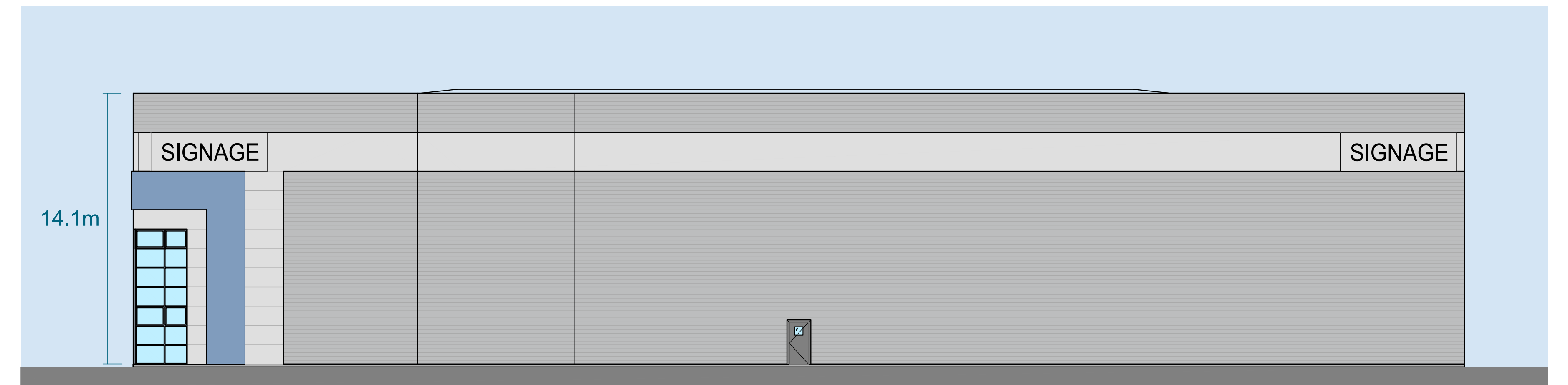
North Elevation
