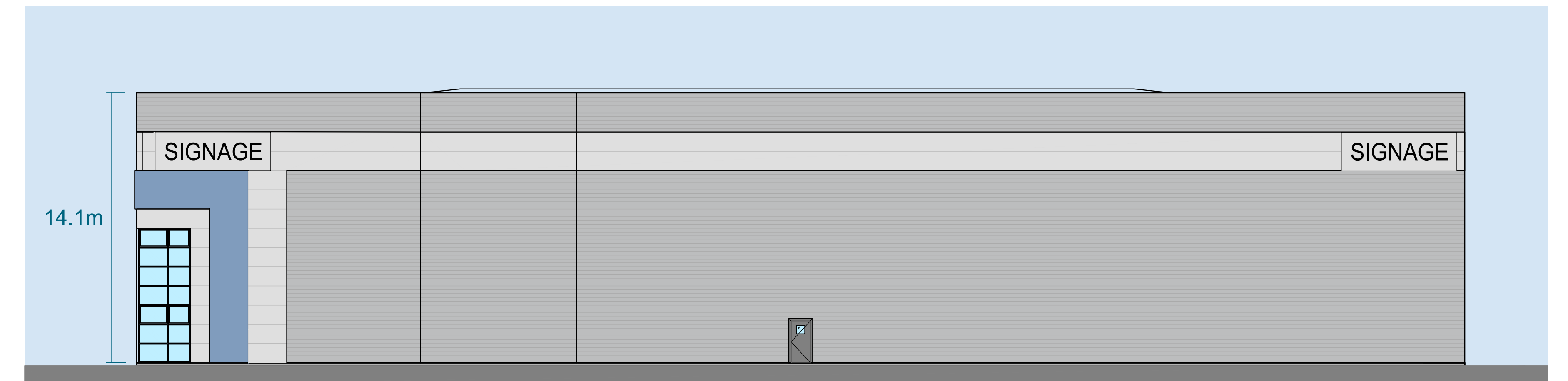
North Elevation
