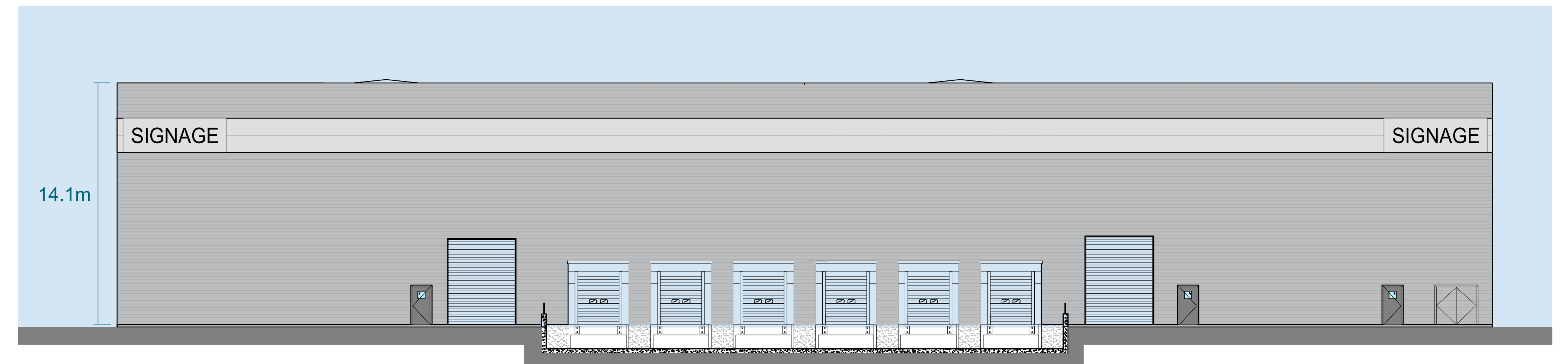
West Elevation
