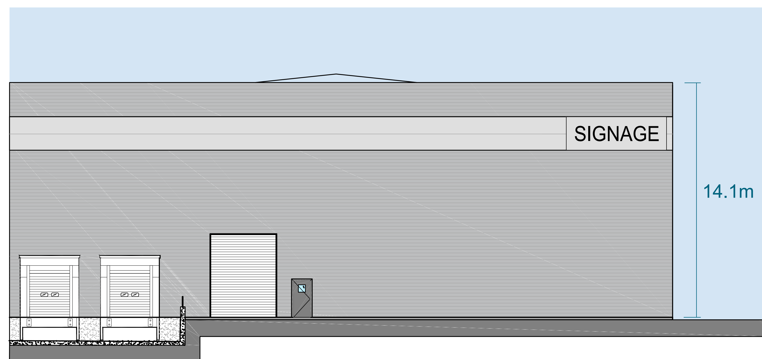
West Elevation
