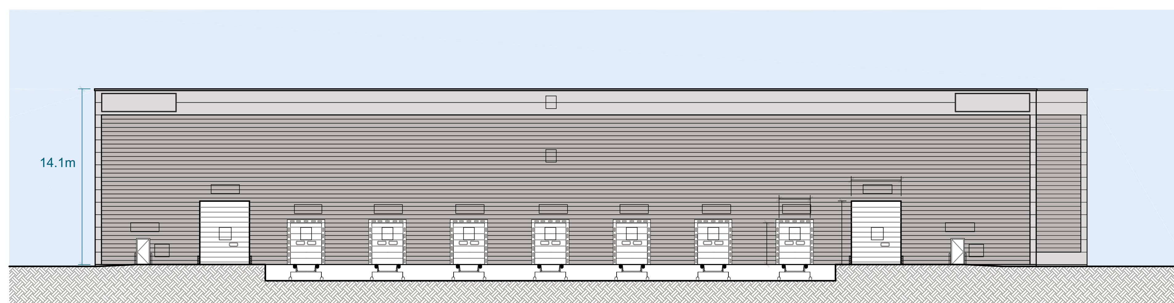
West Elevation
