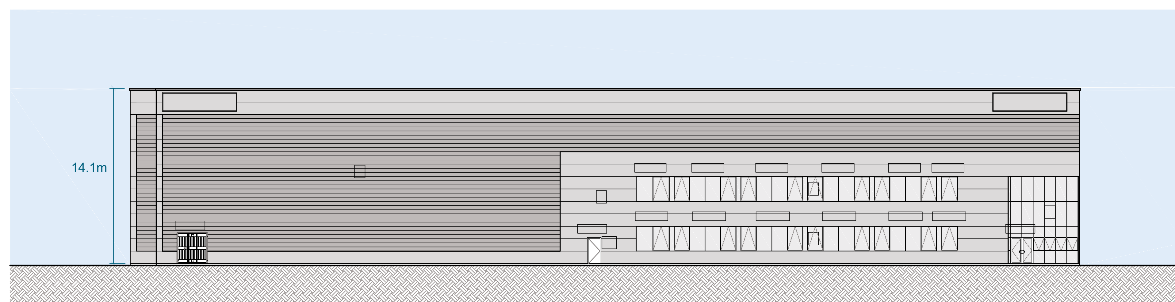
South Elevation
