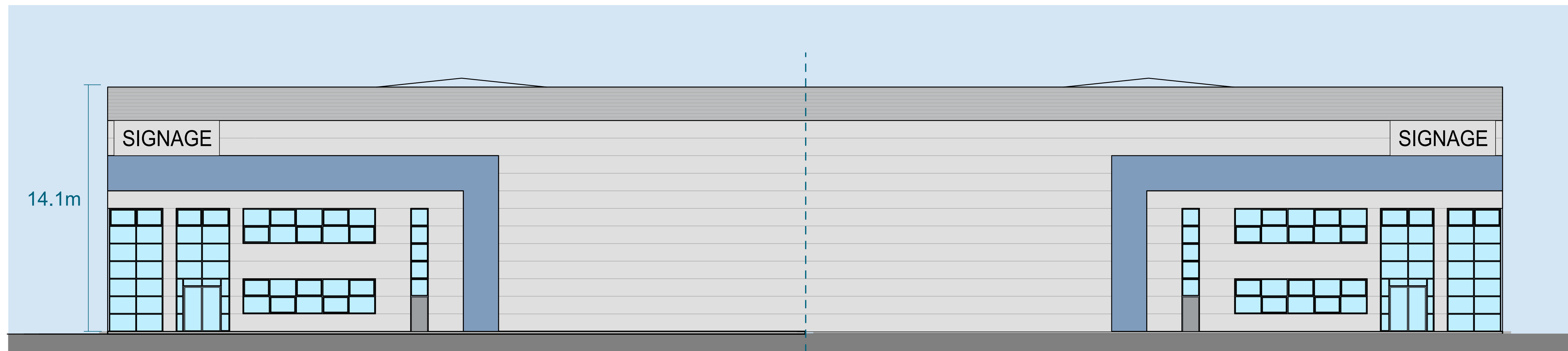
East Elevation
