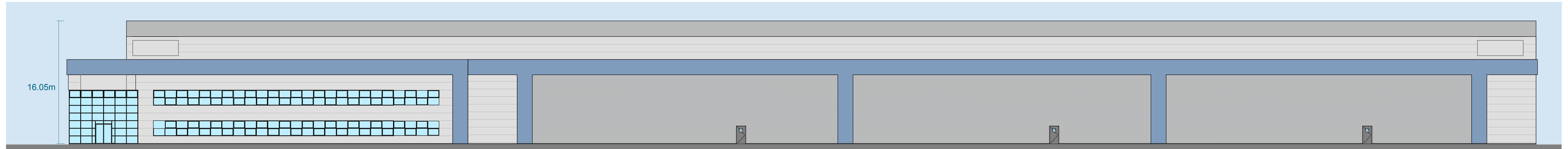
East Elevation
