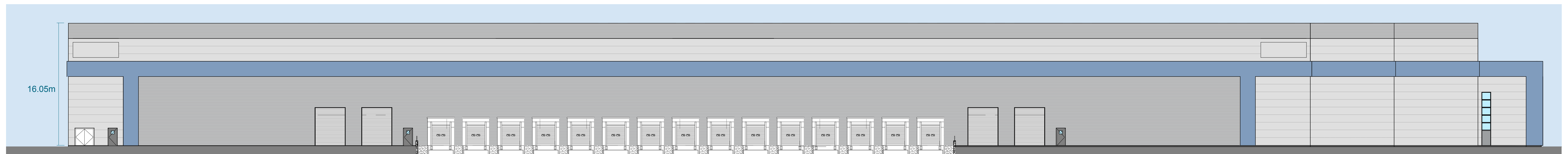
West Elevation
