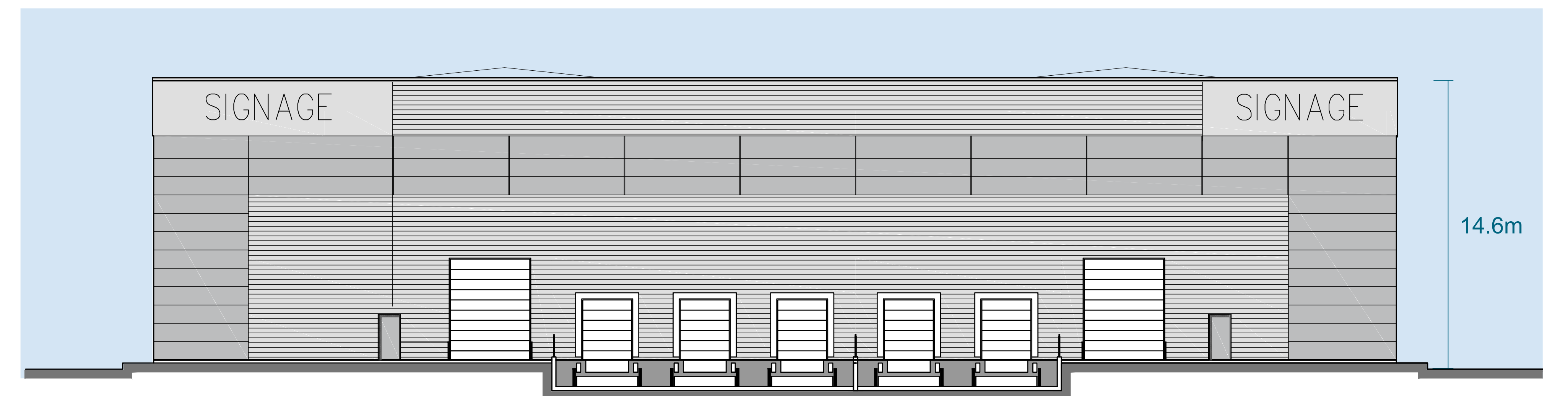
North Elevation
