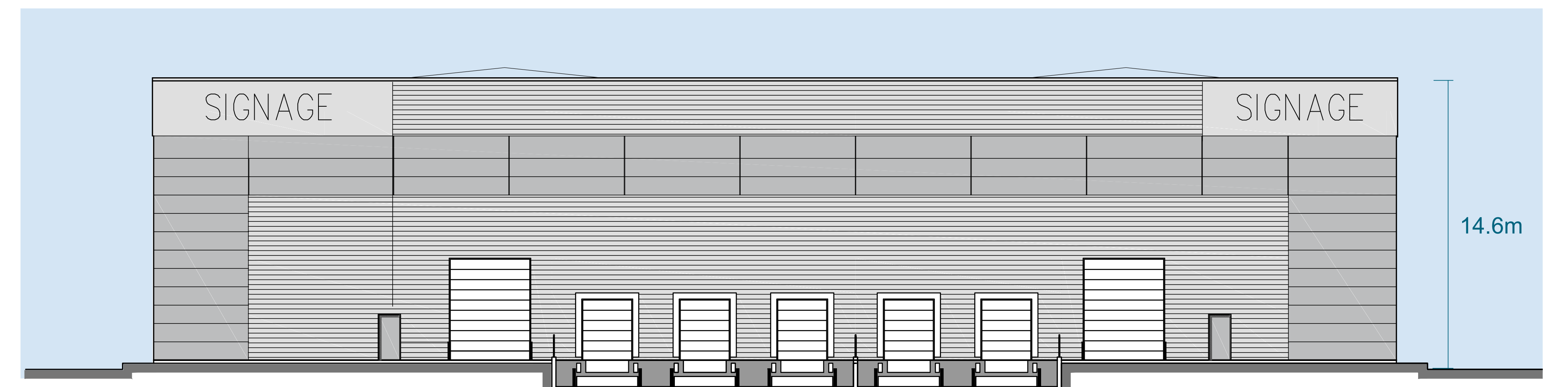
North Elevation
