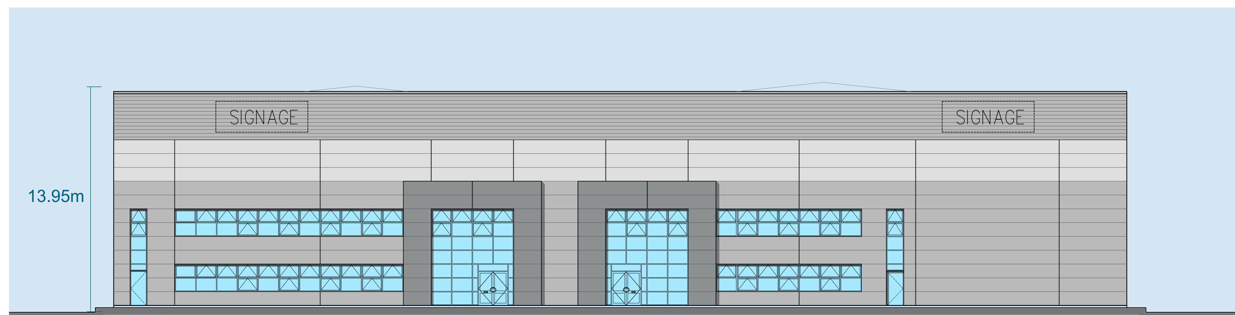
South Elevation
