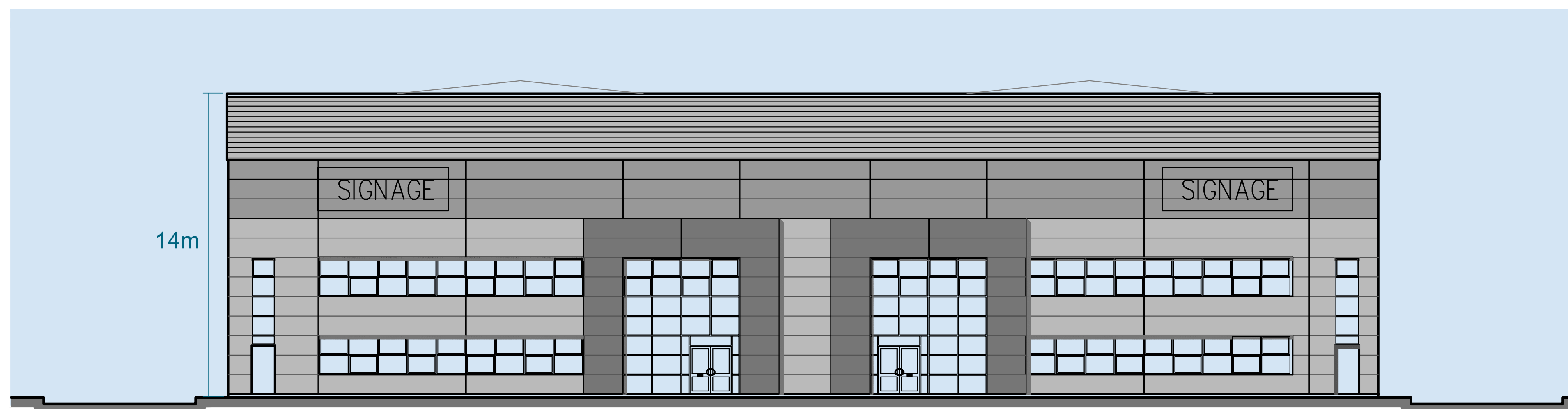
South Elevation
