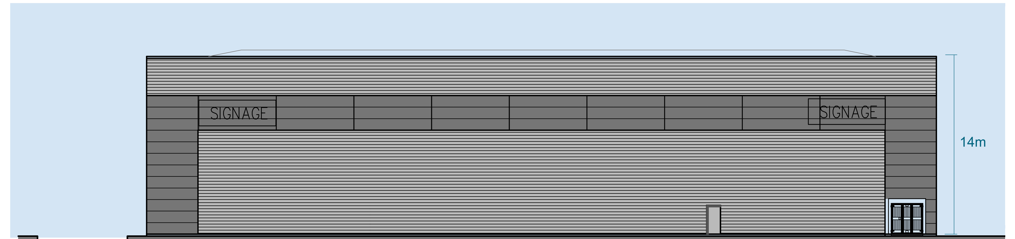
East Elevation
