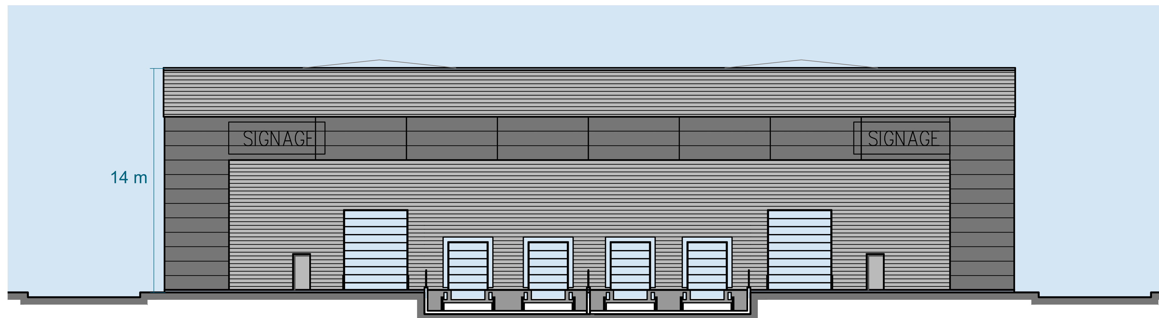
North Elevation
