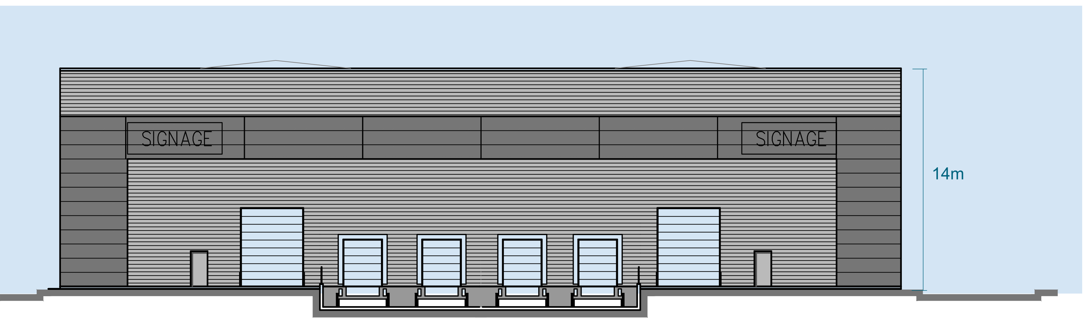
North Elevation
